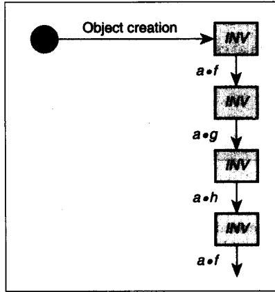
Figure 5. The invariant in an object's life cycle.
