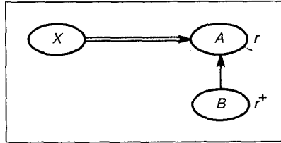
Figure 8. Redefinition of a routine under contract.
